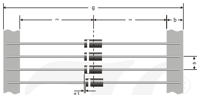
Tape dimensions – Gurtmaße [mm]
