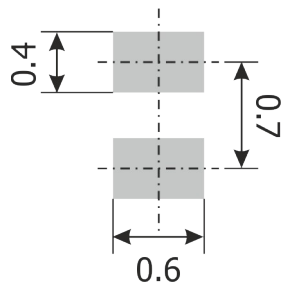
DFN1006-2 (SOD-882)
