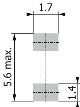
MiniMelf DO-213 AA/SOD-80C
