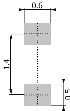
SOD-523
