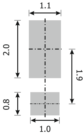
Power SOD-323
