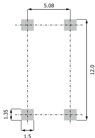
DIL
