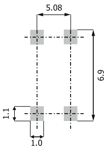
Mini-DIL
