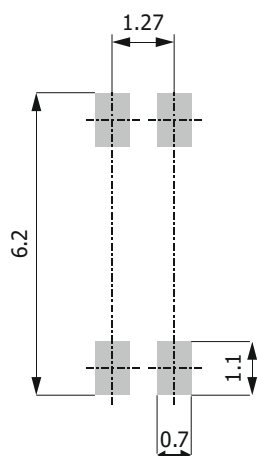
Micro-DIL
