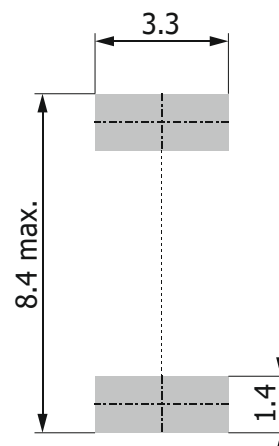
SMC DO-214 AB
