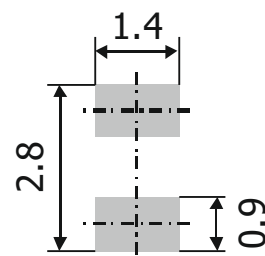
MicroMelf SOD-106C
