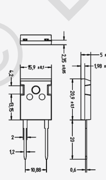
TO-247-2L
