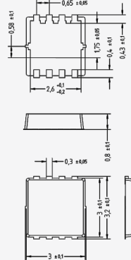
QFN3x3
