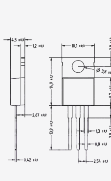
TO-220AB
