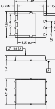
QFN5x6
