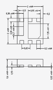
QFN2x2
