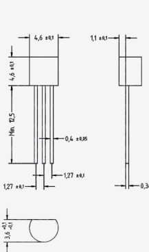
TO-92
