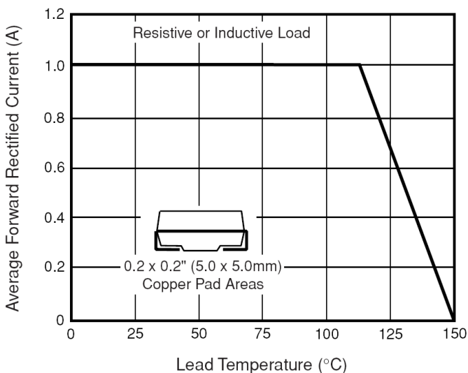
Fig. 2: Marketing trick No. 2 – Referencing to Lead Temperature gives better looking curve
