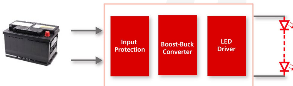
Block diagram for typical automotive lighting applications
