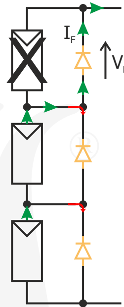
Bypass operation
