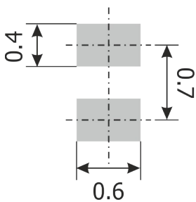
DFN1006-2 (SOD-882)
