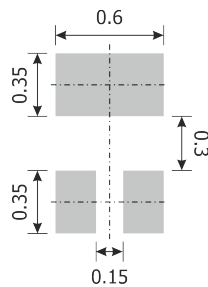
DFN1006-3 (SOT-883)
