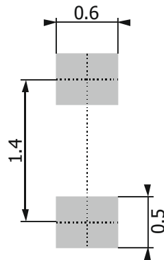
SOD-523
